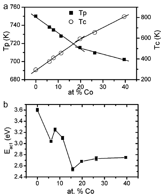
Fig. 1. Curie temperature of the as-cast alloys ( T_c ), peak temperatures of the 1st DSC event ( T_p ) (a) and apparent activation energies of the nanocrystallization process vs. at.% Co content in the alloys (b).
