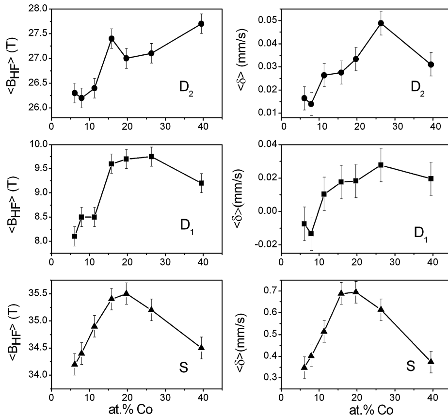
Fig. 9. Average hyperfine magnetic field, \langle B_{HF} \rangle , and average isomer shift \langle \delta \rangle , of the amorphous phase ( D_1 ), the interface ( D_2 ) and the crystalline sextets ( S ) of nanocrystalline samples as a function of the Co content of the alloy.
