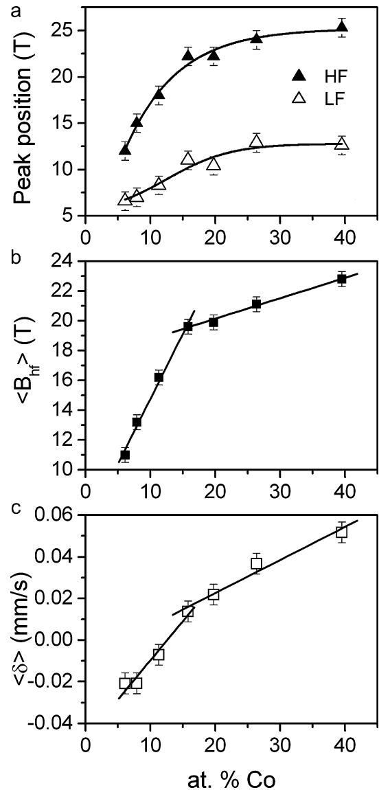
Fig. 6. Peak position of high field component (HF) and low field component (LF) of the hyperfine field distributions (a); the average hyperfine magnetic field (b) and the average isomer shift (c), corresponding to as-quenched samples as a function of the Co content.
