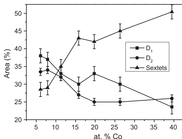
Fig. 8. Area of the amorphous phase ( D_1 ), the interface ( D_2 ) and the crystalline sextets ( S ) of nanocrystalline samples as a function of the Co content.
