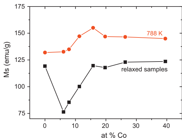
Fig. 10. Saturation magnetization, M_s , vs. at.% Co content in the alloys for relaxed and nanocrystalline samples.
