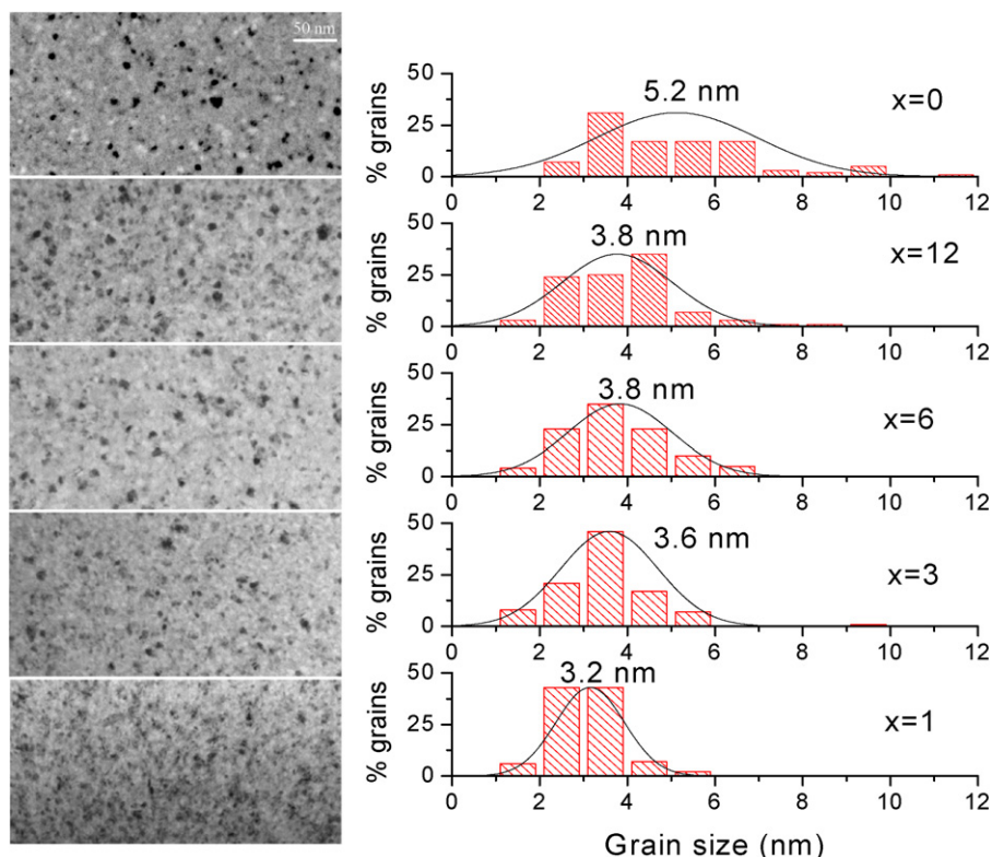
Fig. 4. TEM bright field images obtained for samples of 0 at.% Co and x = 12, 6, 3, 1 alloys heated up to the end of their first crystallization event (left) and their corresponding distribution of grain sizes (right).
