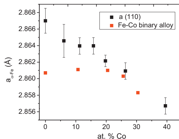
Fig. 3. Lattice parameter of the \alpha\text{-FeCo(Mo)} phase at the end of the first DSC event as a function of the Co content of the alloy. Values of those of FeCo binary alloy are included for comparison.
