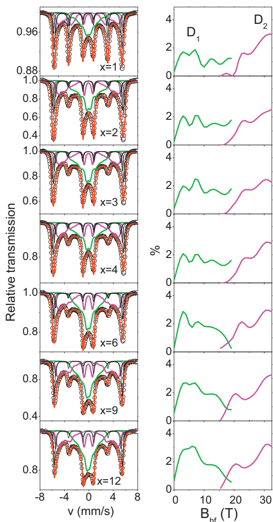
Fig. 7. Mössbauer spectra of partially crystallized samples, after heated up to the end of the first DSC event, taken at 300 K, and their hyperfine field distributions corresponding to the amorphous phase ( D_1 ) and the interface ( D_2 ).
