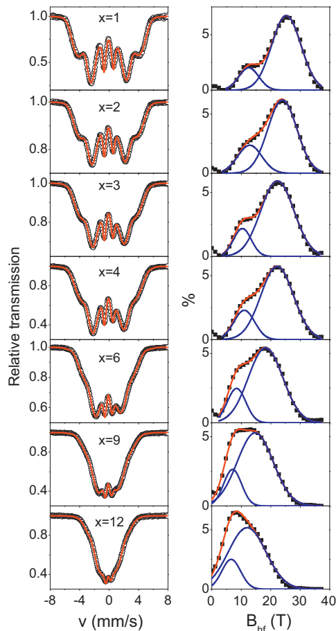
Fig. 5. Mössbauer spectra of as-quenched samples taken at 300 K and their corresponding hyperfine field distributions.
