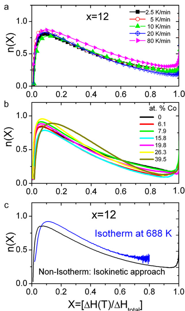
Fig. 2. n(X) from DSC scans of x=12 alloy taken at different heating rates (a). n(X) from DSC scans of the studied alloys taken at 10 K/min (b). Comparison between isothermal TMG (shorter line) and non-isothermal DSC (taken at 2.5 K/min) results for the x=12 alloy (c).
